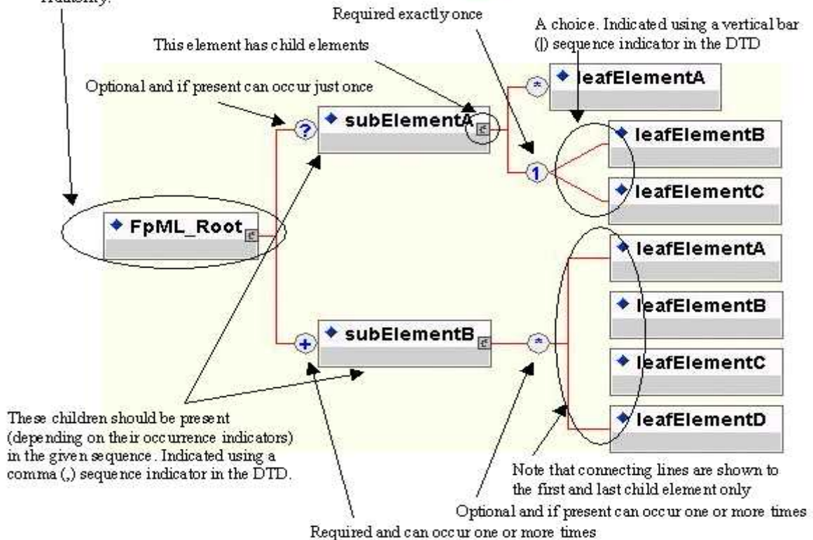
Figure 5.1: Graphical Representation of a DTD
